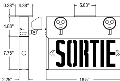
Type RMSM - PAR18 Thermoplastic
