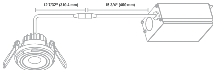
LED Module and Driver
