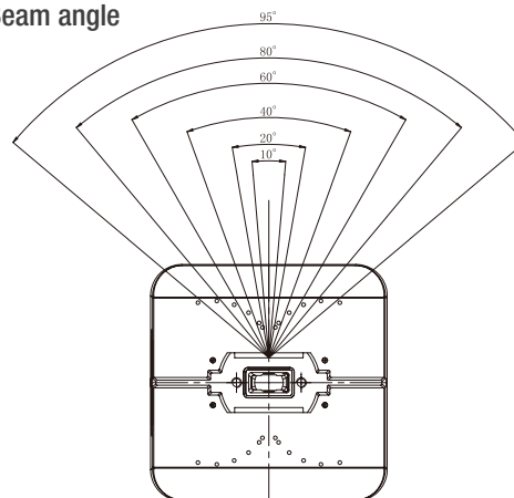
Beam angle
