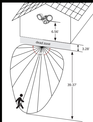
MOTION SENSOR DETECTION COVERAGE
